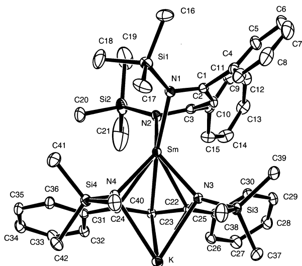
Fig. 15. The molecular structure of [\{K(\mu\text{-J})\text{SmJ}\}_2] ( 26 ), showing a single unit of the dimer.
