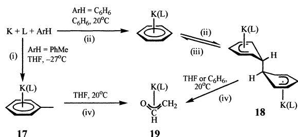
Scheme 6. Synthesis of the crystalline complexes 17 – 19 from K, ([18]crown-6) (= L) and PhMe or C 6 H 6 .
