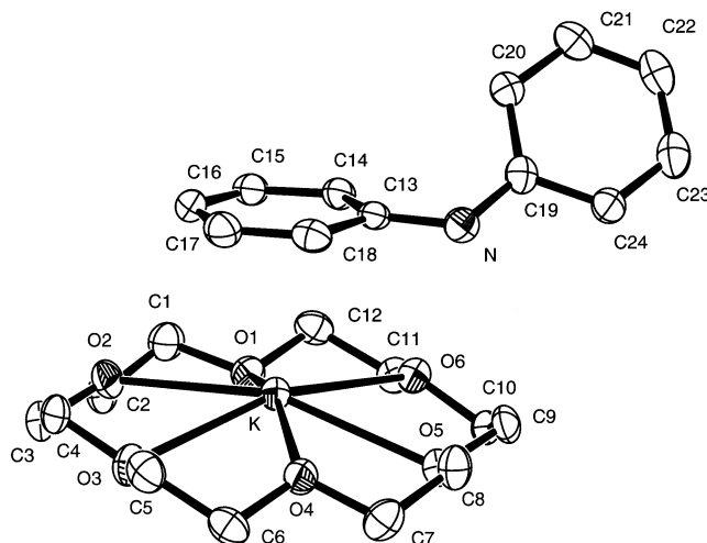
Fig. 14. The molecular structure of [K(NPh 2 ) 2 ([18]crown-6)] ( 25 ).
