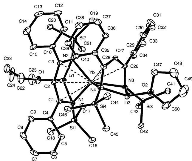
Fig. 16. The molecular structure of [\{\text{Li}(\text{thf})_2\text{Yb}(\text{J})_2\}] ( 27 ).
