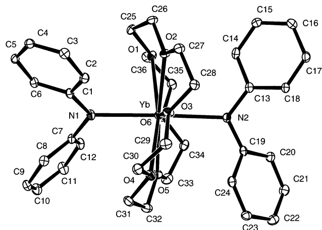
Fig. 13. The molecular structure of [Yb(NPh 2 ) 2 ([18]crown-6)] ( 23 ).
