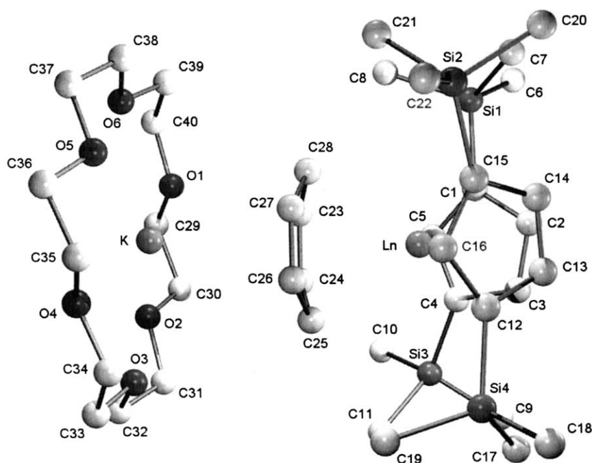
Fig. 2. The molecular structure of the isostructural compounds [\text{K}(\text{[18]crown-6})][\text{LnCp}''_2(\eta^2\text{-C}_6\text{H}_6\text{-1,4})] 5a , 5b and 5d .
