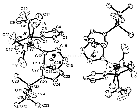
Fig. 5. The structure of the anion of [K([18]\text{crown-6})(\eta^2\text{-PhMe})_2][(CeCp^*_3)_2(\mu\text{-H})] ( 9b ) ( \mu\text{-H} not located).
