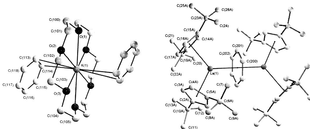
Fig. 3. The structure of [\text{K}([18]\text{crown-6})(\eta^2\text{-C}_6\text{H}_6)_2][(\text{LaCp}^x_2)_2(\mu\text{-}\eta^6\text{-}\eta^6\text{-C}_6\text{H}_6)] ( 7b ).
